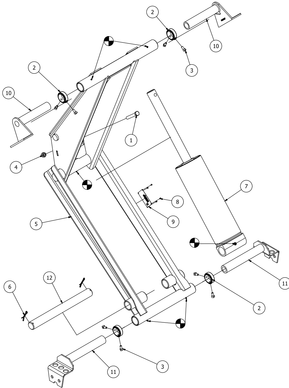
CS615T Parts List (refer to engineering drawing A12675)
