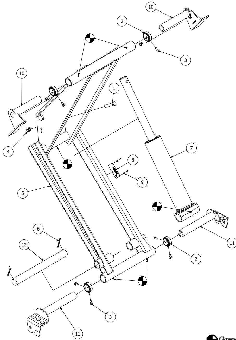
CS415T Parts List (refer to engineering drawing A12673)
