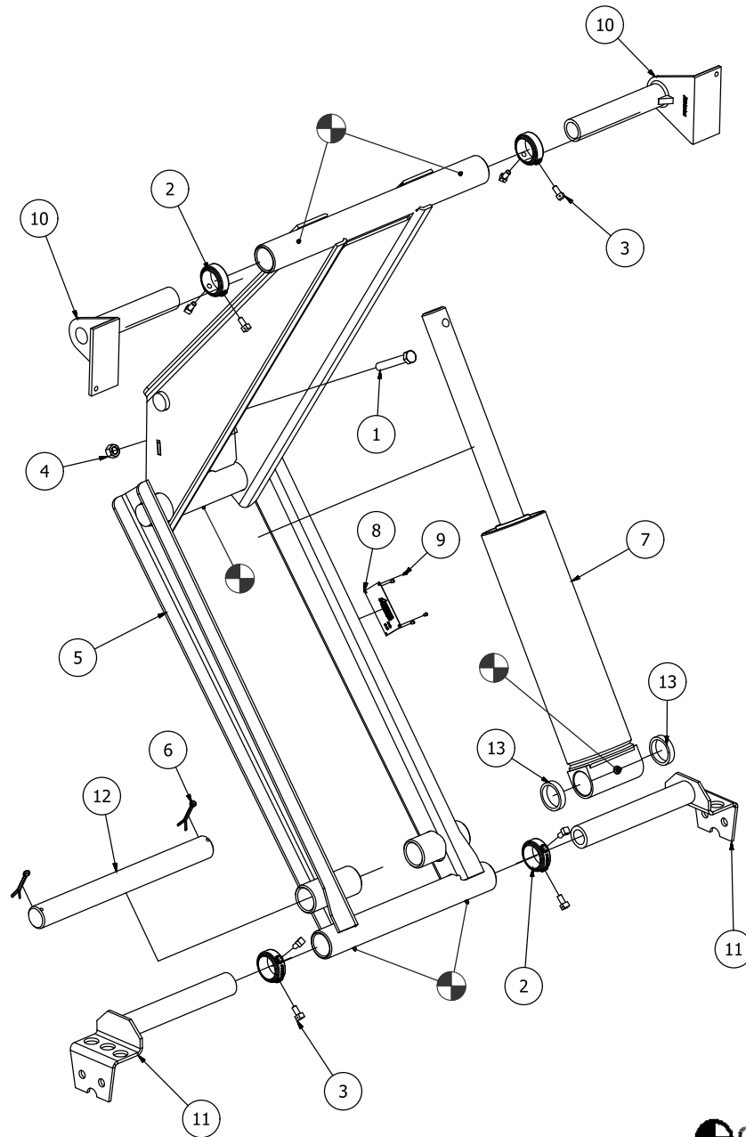
CS515T Parts List (refer to engineering drawing A12674)
