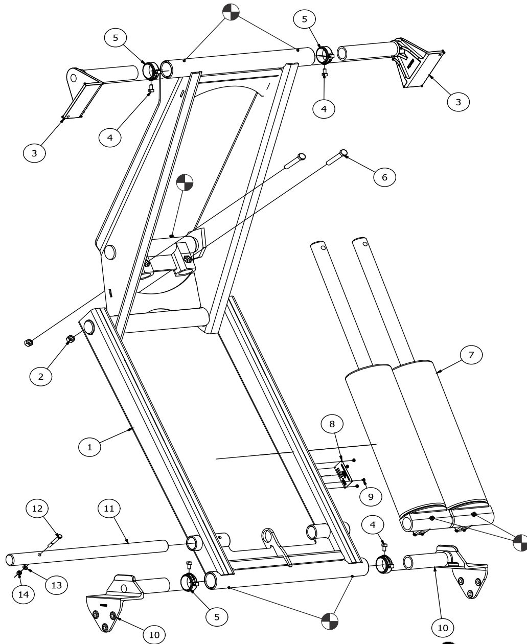
CS6620T Parts List (refer to engineering drawing A12679)
